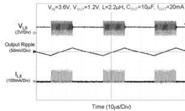
Fig. 18 PSM Operation
