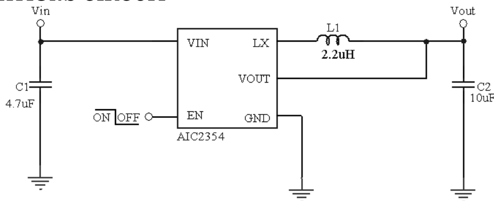
Fig. 1 Fixed Step-Down DC/DC Converter
