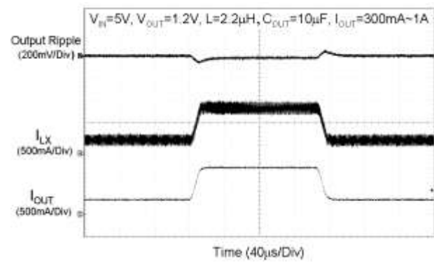
Fig. 16 Load Transient Response
