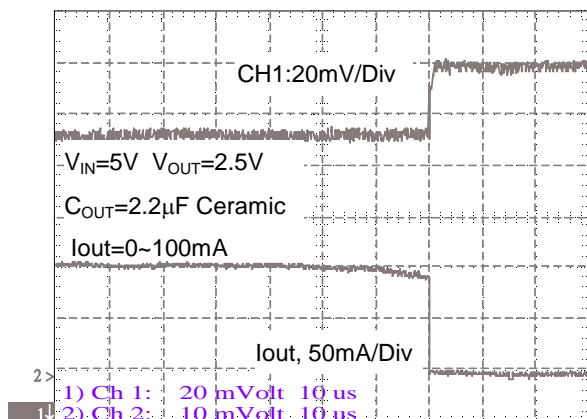
Fig. 18 Load Transient Response
