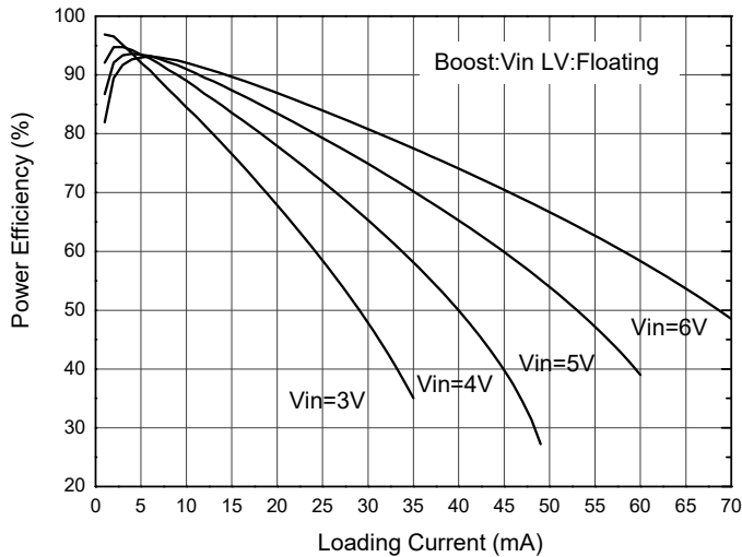
Fig. 7 Power Efficiency vs. Load Current
