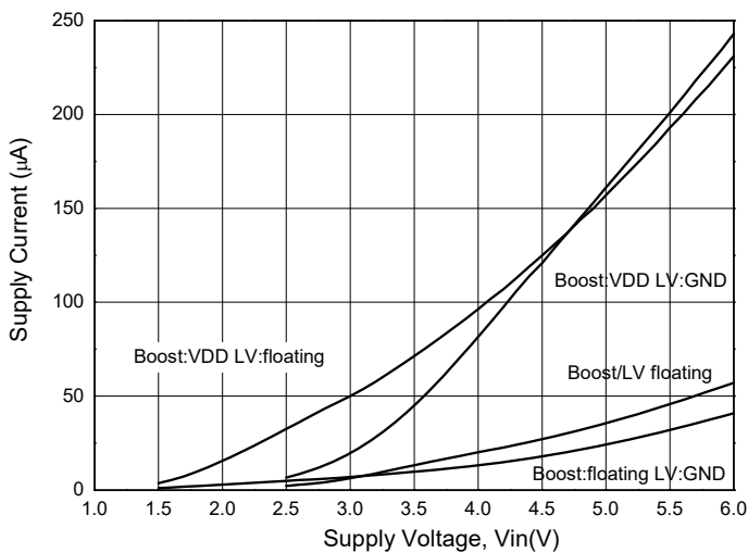
Fig. 11 Supply Current vs. Supply Voltage
