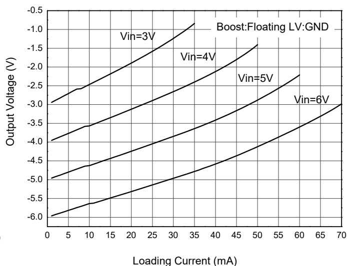
Fig. 4 Output Voltage vs. Load Current
