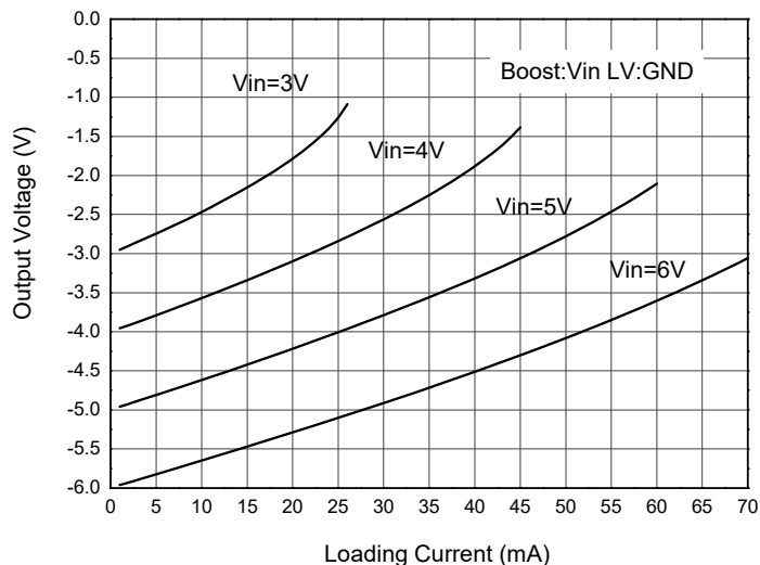
Fig. 2 Output Voltage vs. Load Current
