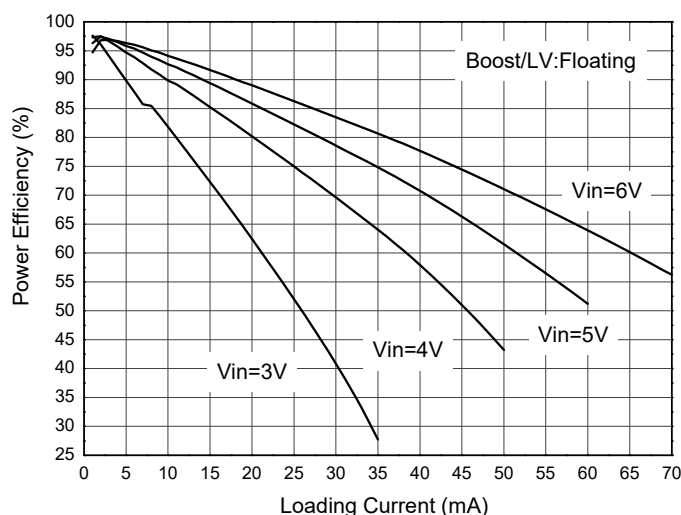
Fig. 5 Power Efficiency vs. Load Current
