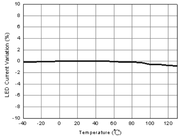
Fig.4 LED current vs. Temperature
