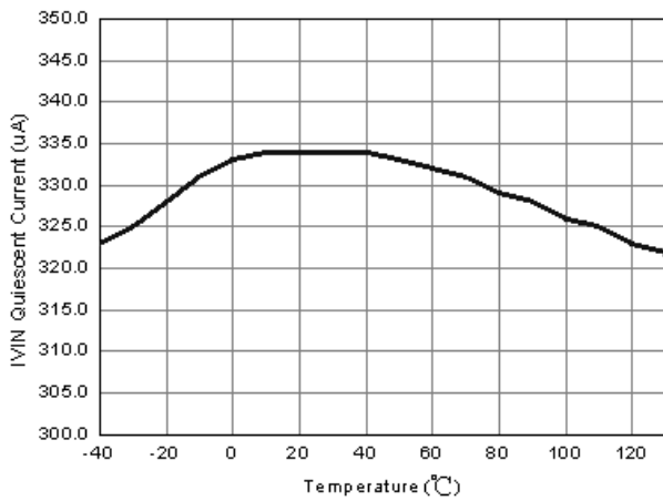
Fig.3 Quiescent Current
