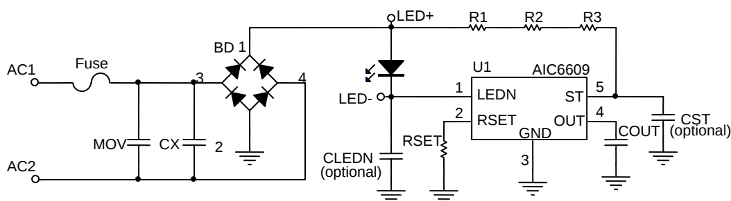
Fig.2. Typical Application Circuit for TO252-5
