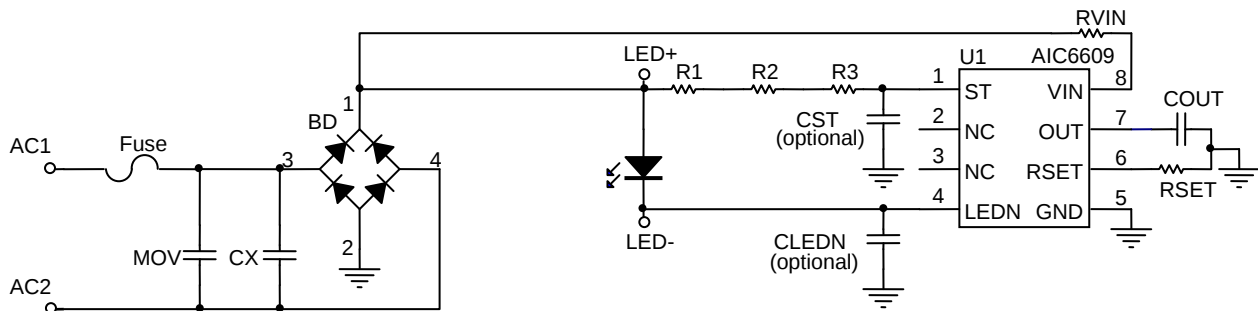
Fig.1. Typical Application Circuit for SOP-8
