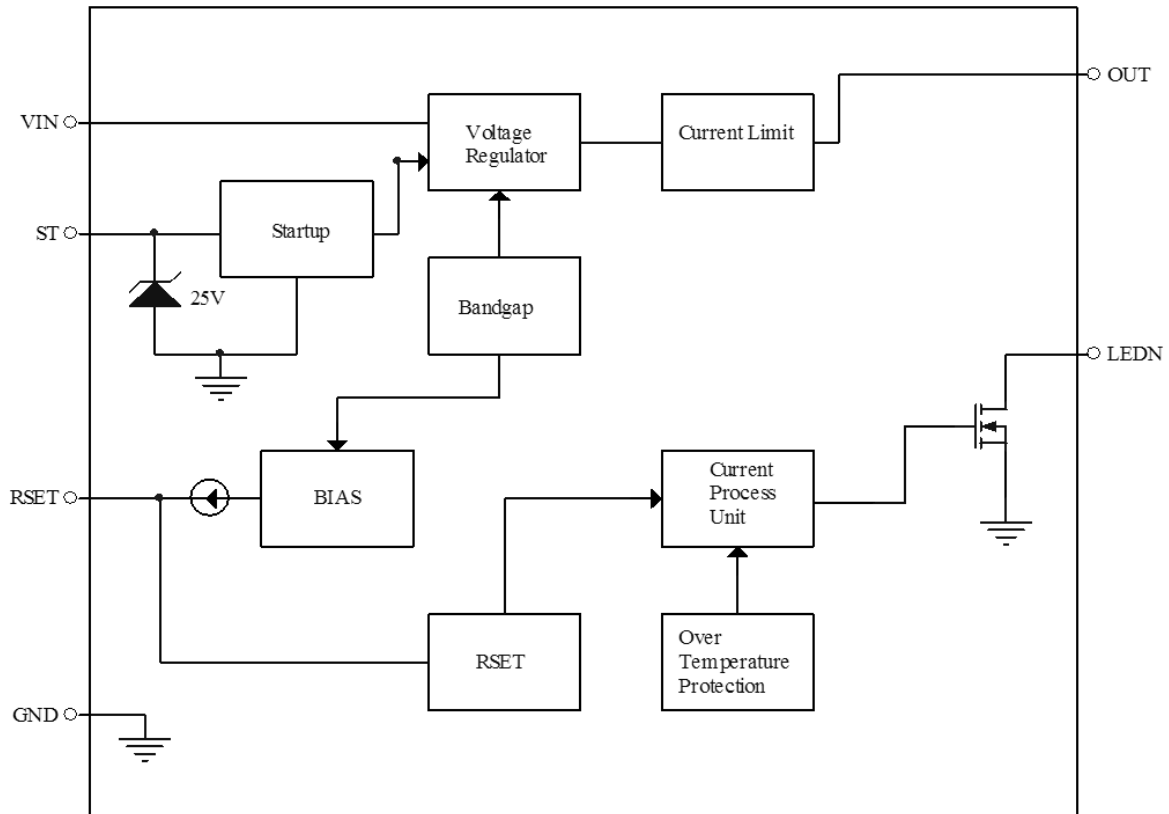
Functional Block Diagram of AIC6609
