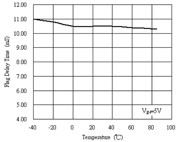
Fig. 8 Flag Delay Time vs. Temperature
