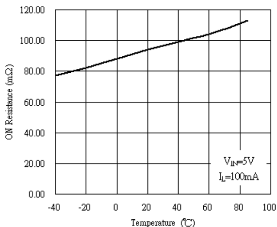
Fig. 2 ON Resistance vs. Temperature
