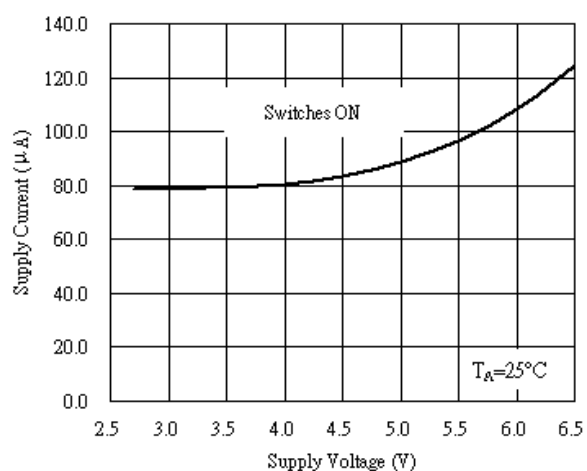
Fig. 3 ON-State Supply Current vs. Supply Voltage
