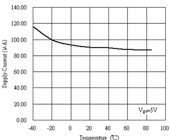
Fig. 4 ON-State Supply Current vs. Temperature
