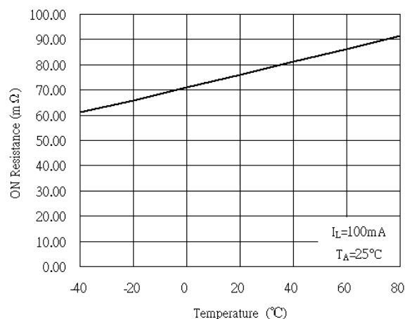
Fig. 2 ON Resistance vs. Temperature
