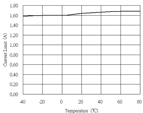
Fig. 6 Current Limit vs. Temperature
