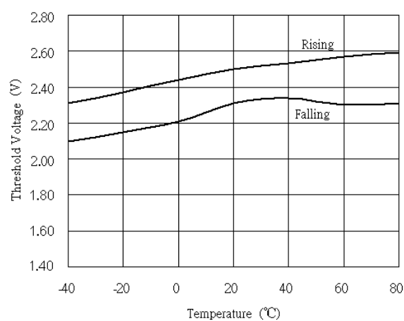
Fig. 10 UVLO Threshold Voltage vs. Temperature
