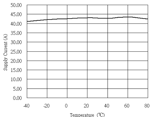
Fig. 4 ON State Current vs. Temperature
