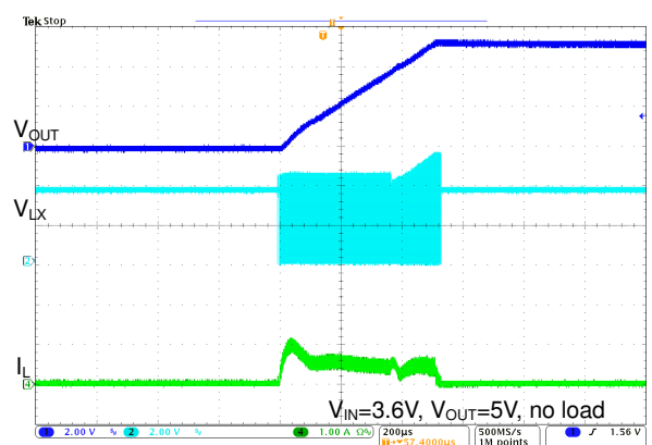
Fig. 10 Start-up Waveform
