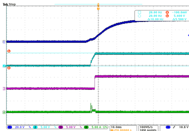
Fig. 9 V_{IN} Power On ( V_{IN}=36V , V_{OUT}=5V , I_{OUT}=100mA )
