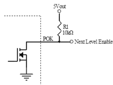
Fig. 15 Power Good Circuit
