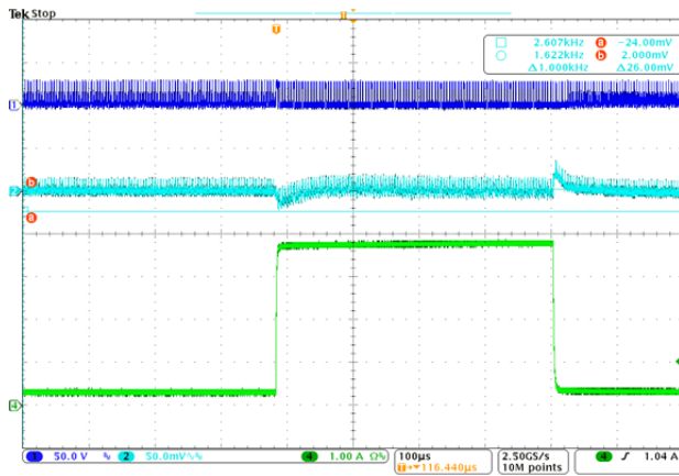
Fig. 13 Load Transient ( V_{IN}=24V , V_{OUT}=5V , I_O=0.4-3.6A )
