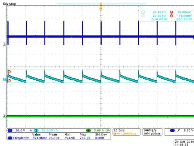
Fig. 7 Output Ripple ( V_{IN}=36V , V_{OUT}=12V , I_{OUT}=1mA )
