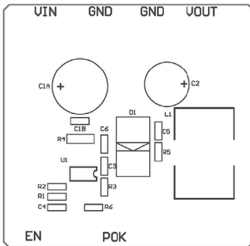
Fig. 18 Top Component Placement
