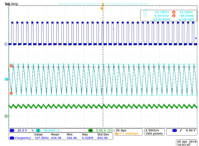
Fig. 8 Output Ripple ( V_{IN}=36V , V_{OUT}=12V , I_{OUT}=4A )
