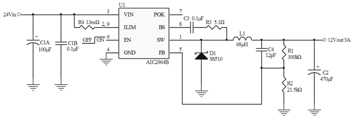
Fig. 20 AIC2964B Application Circuit for 12V/3A Output Application
