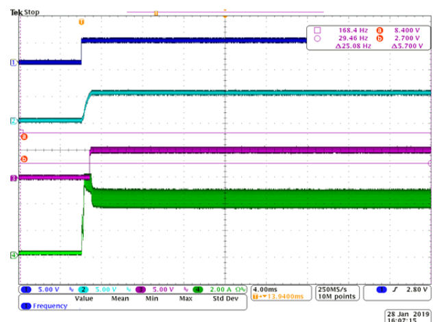
Fig. 12 Enable On ( V_{IN}=36V , V_{OUT}=5V , I_{OUT}=4A )
