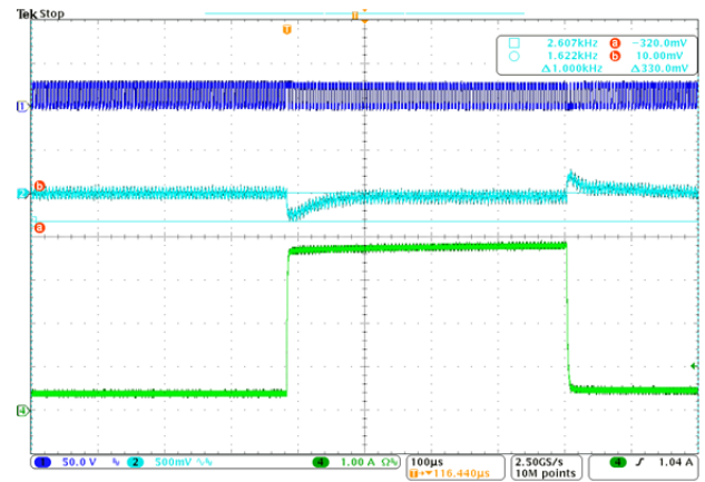
Fig. 14 Load Transient ( V_{IN}=24V , V_{OUT}=12V , I_O=0.4-3.6A )
