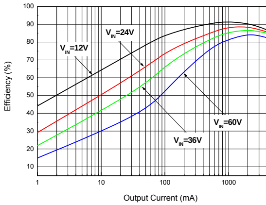
Fig. 1 Efficiency vs. Output Current ( V_{OUT}=5V )
