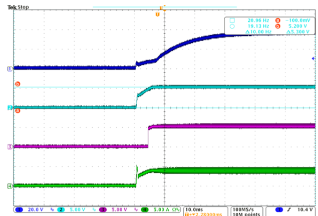
Fig. 10 V_{IN} Power On ( V_{IN}=36V , V_{OUT}=5V , I_{OUT}=4A )
