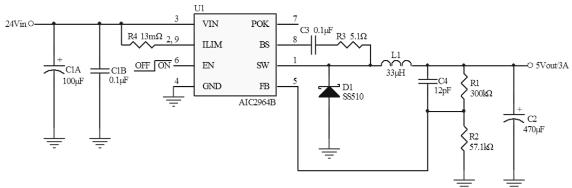
Fig. 19 AIC2964B Application Circuit for 5V/3A Output Application
