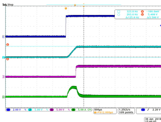
Fig. 11 Enable On ( V_{IN}=24V , V_{OUT}=5V , I_{OUT}=100mA )
