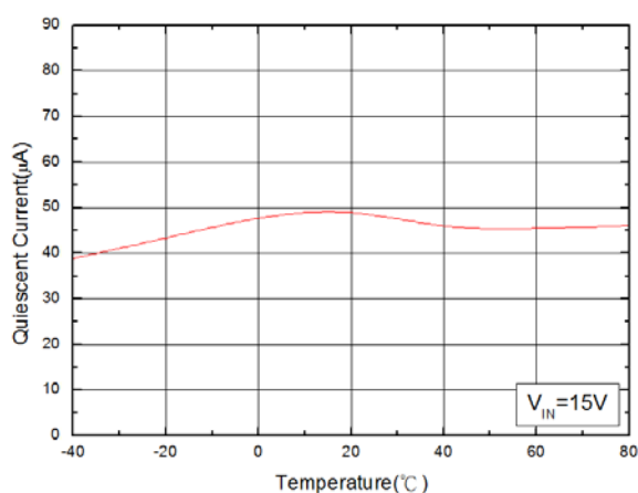
Fig. 11 Quiescent Current vs. Temperature
