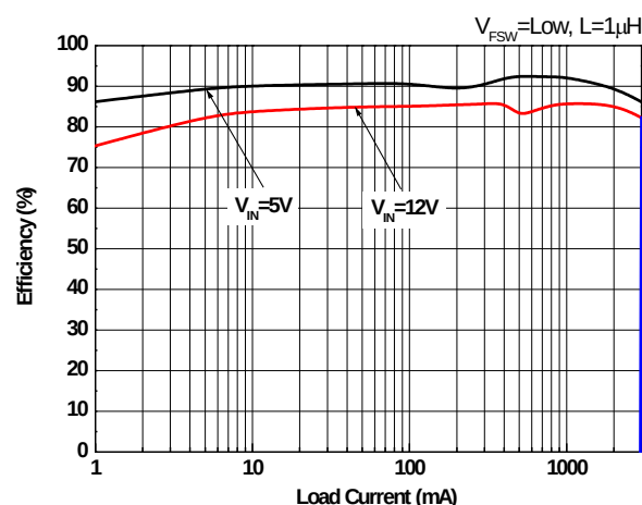
Fig. 5 Efficiency vs. Load Current ( V_{OUT}=3.3\text{V} )
