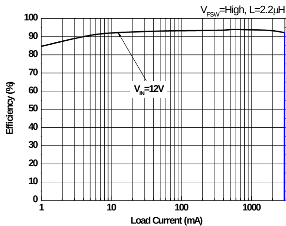
Fig. 1 Efficiency vs. Load Current ( V_{OUT}=5\text{V} )
