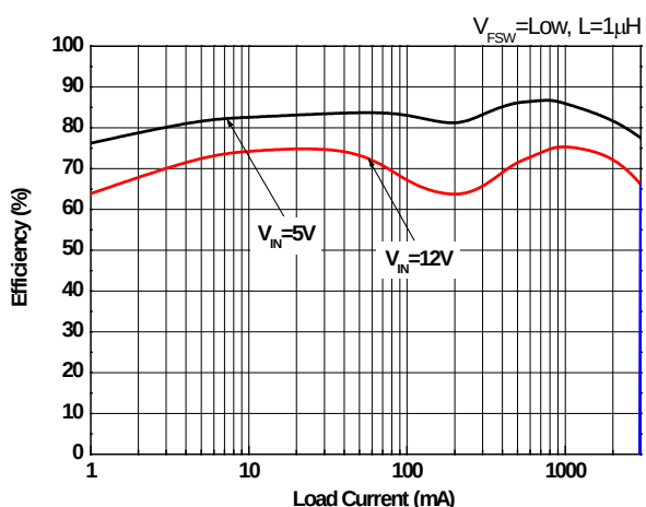
Fig. 6 Efficiency vs. Load Current ( V_{OUT}=1.8\text{V} )
