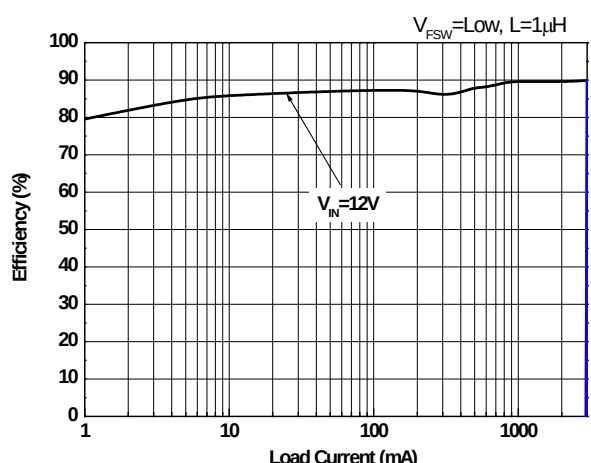
Fig. 4 Efficiency vs. Load Current ( V_{OUT}=5\text{V} )
