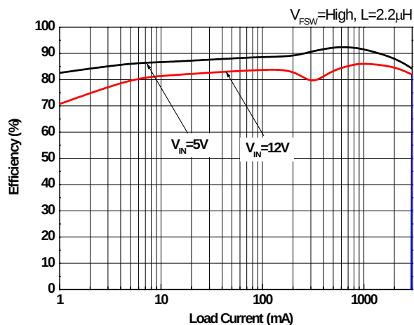
Fig. 3 Efficiency vs. Load Current ( V_{OUT}=1.8\text{V} )
