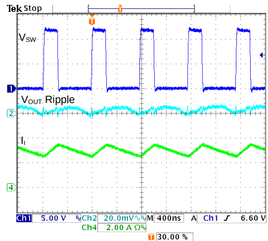
Fig. 14 Output Ripple ( V_{IN}=12V , V_{OUT}=3.3V , I_{OUT}=3A )
