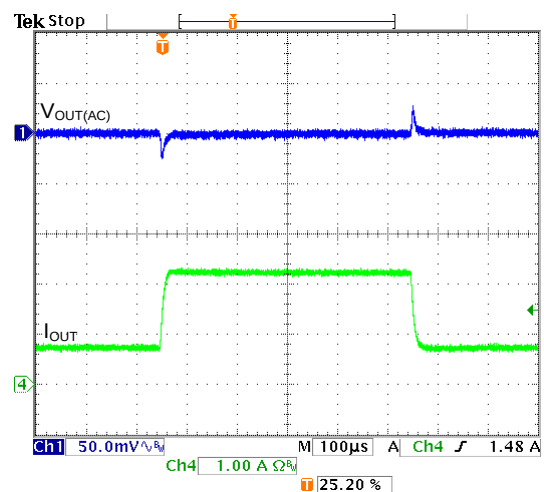
Fig. 18 Load Transient ( V_{IN}=12V , V_{OUT}=3.3V , I_o=0.75-2.25A )
