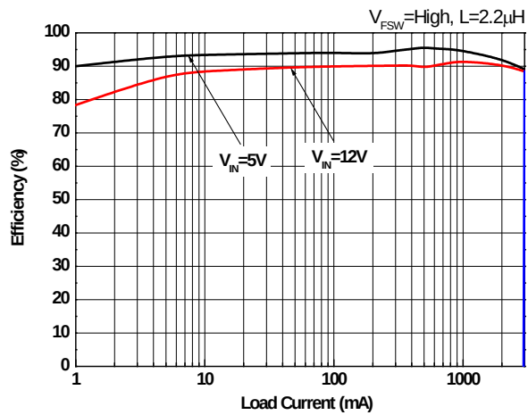
Fig. 2 Efficiency vs. Load Current ( V_{OUT}=3.3\text{V} )
