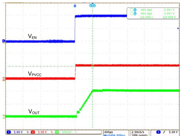
Fig. 10 Star_Up at V IN =12V, V OUT =1.05V, I OUT =0A
