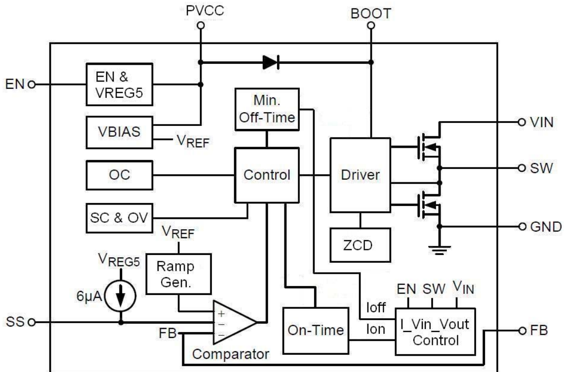
Functional Block Diagram of AIC2865
