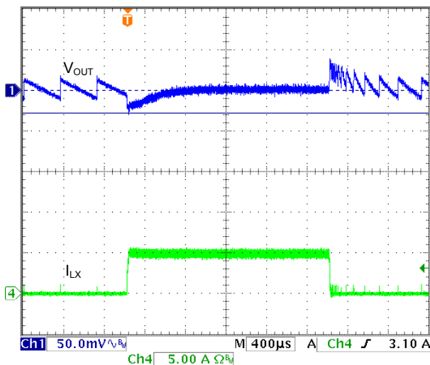
Fig. 9 V IN =12V, V OUT =1.05V, I OUT =0A to 5A
