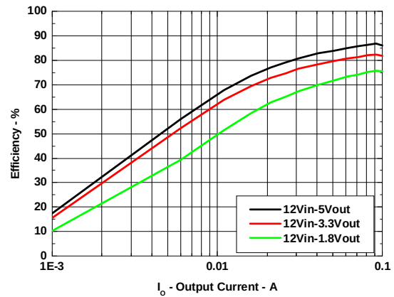
Fig. 4 Light Load Efficiency vs. Output Current
