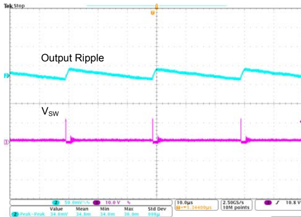
Fig. 7 Output Ripple at V IN =12V, V OUT =1.05V, I OUT =30mA Fig. 8 Output Ripple at V IN =12V, V OUT =1.05V, I OUT =5A
