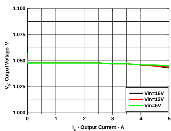
Fig. 6 Output Voltage vs. Output Current
