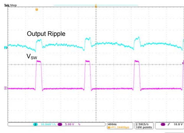
Fig. 7 Output Ripple at V IN =12V, V OUT =1.05V, I OUT =30mA Fig. 8 Output Ripple at V IN =12V, V OUT =1.05V, I OUT =5A
