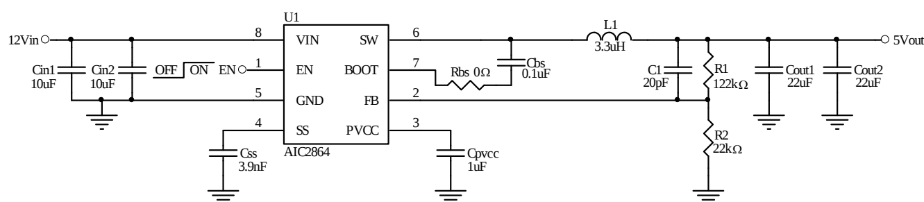
Typical Application Circuit for V IN =12V Condition
