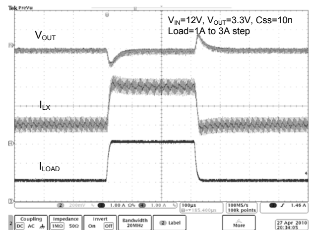
Fig. 6 Load Transient at V_{OUT} = 3.3V , I_{OUT} = 1A to 3A
