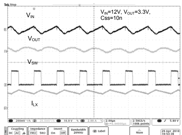
Fig. 10 Stability Waveform at V_{OUT}=3.3V , I_{OUT}=3A
