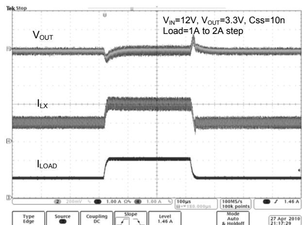
Fig. 6 Load Transient at V_{OUT} = 3.3V , I_{OUT} = 1A to 2A
