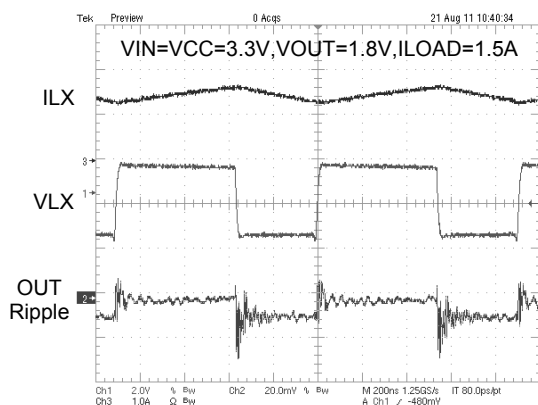
Fig. 3 Switching Waveform
