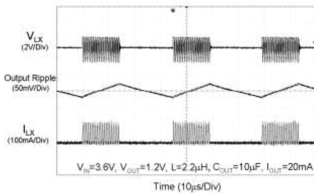
Fig. 17 PSM Operation
