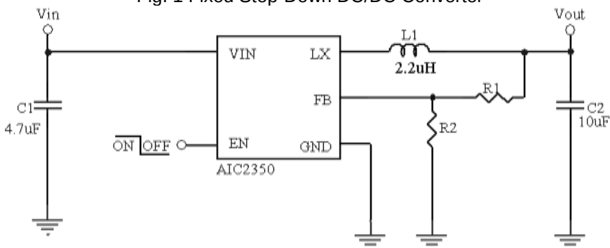
Fig. 2 Adjustable Step-Down DC/DC Converter
