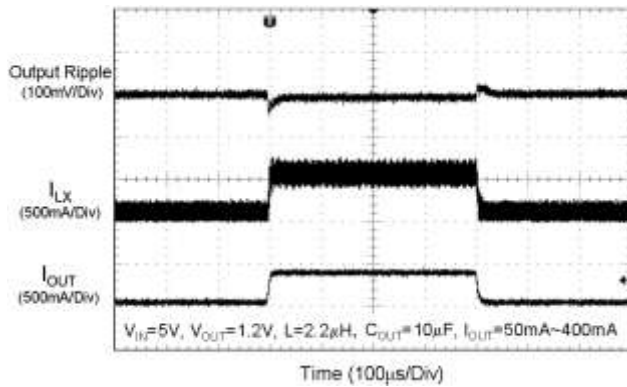
Fig. 15 Load Transient Response
