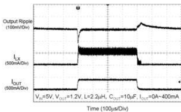
Fig. 13 Load Transient Response
