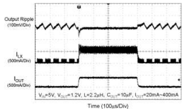
Fig. 14 Load Transient Response
