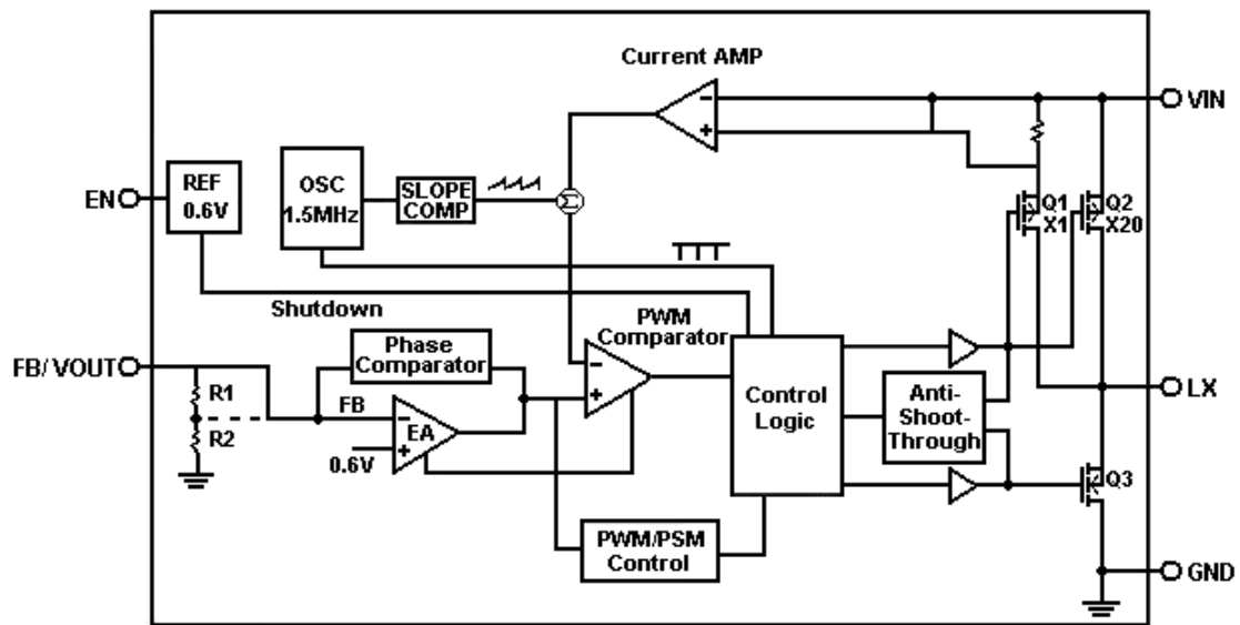
Functional Block Diagram of AIC2350
