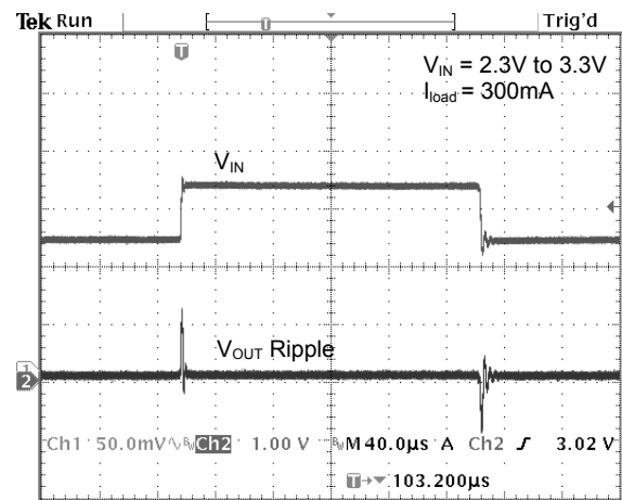
Fig.16 Line Transient Response at V_{OUT}=1.2V , I_{OUT}=300mA
