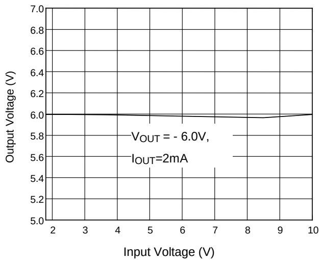
Fig. 7 Line Regulation
