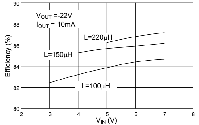
Fig. 8 Efficiency vs. V_{IN}
