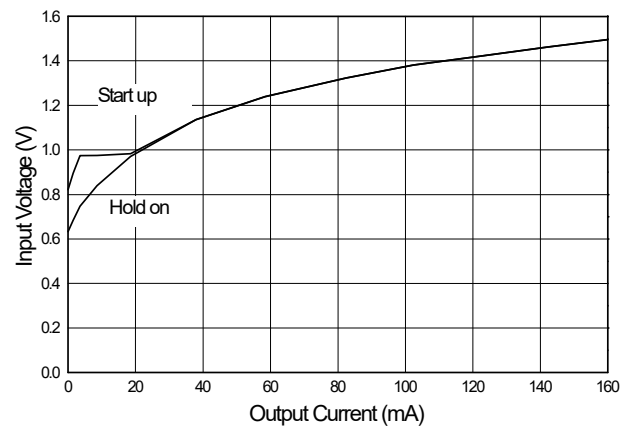
Fig. 12 AIC1639-50 Start-up & Hold-on Voltage (L=33μH)
