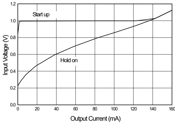
Fig. 11 AIC1639-33 Start-up & Hold-on Voltage (L=33μH)
