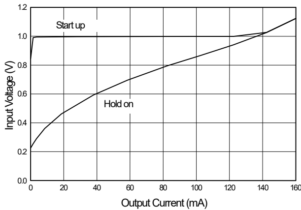
Fig. 13 AIC1639-33 Start-up & Hold-on Voltage (L=33μH)
