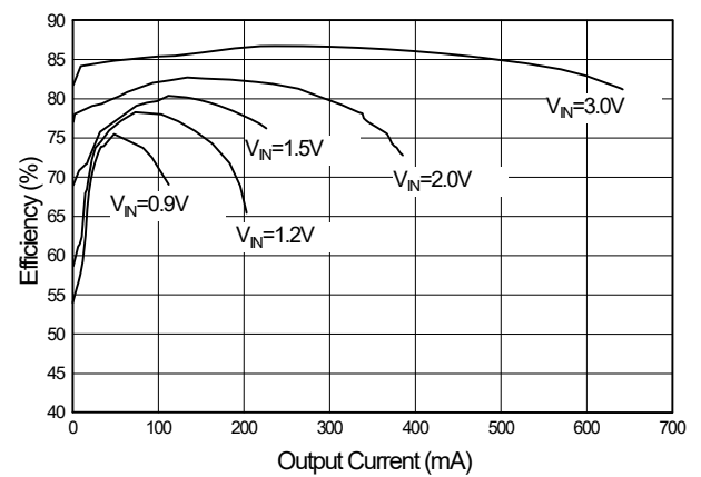
Fig. 8 AIC1639-50 Efficiency ( L=33\mu H )
