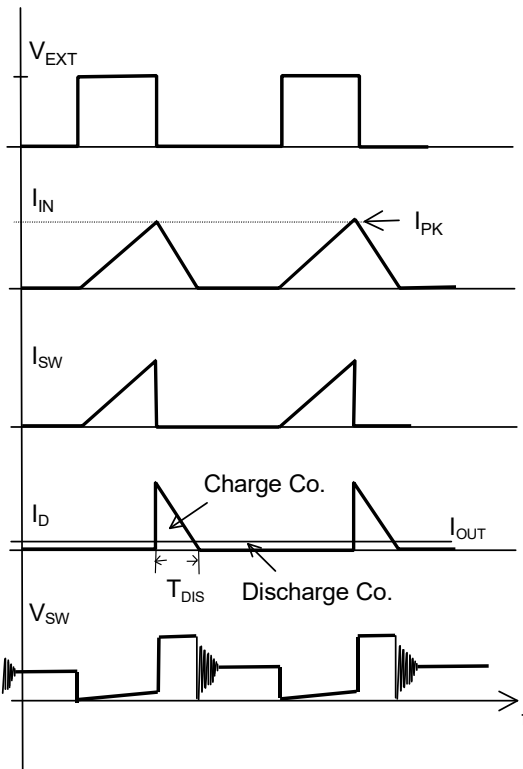
Discontinuous Conduction Mode
