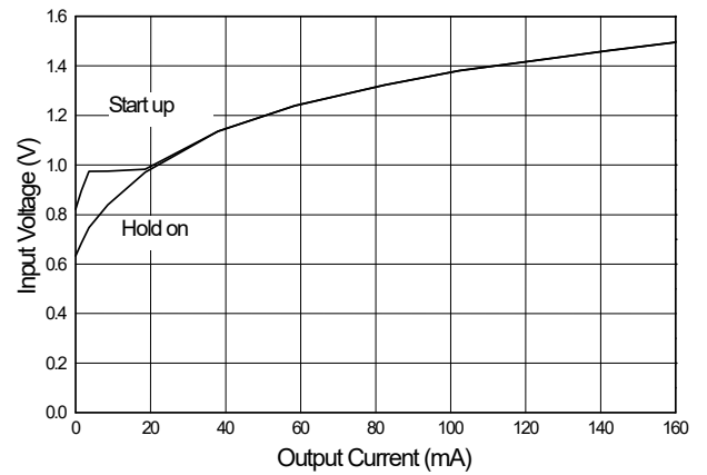
Fig. 14 AIC1639-50 Start-up & Hold-on Voltage (L=33μH)
