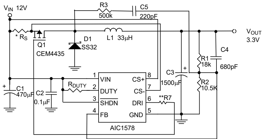
Fig. 12 Step-Down Converter
