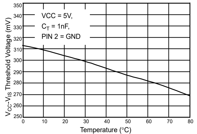
Fig. 4 I_S Threshold Voltage vs. Temperature
