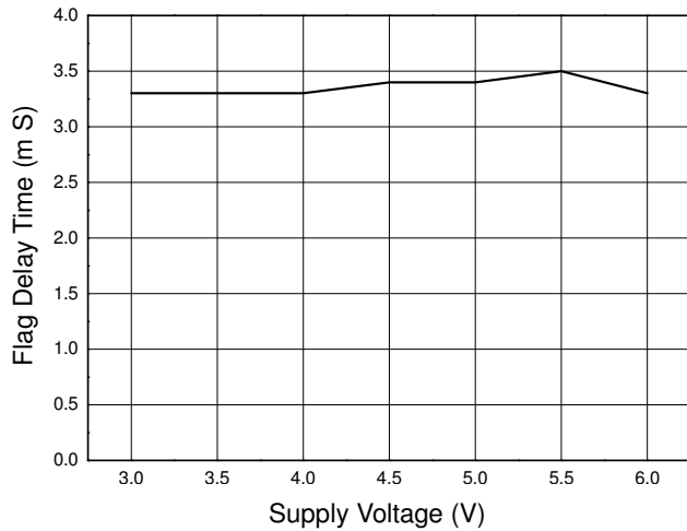
Fig. 13 Flag Delay Time vs. Supply Voltage
