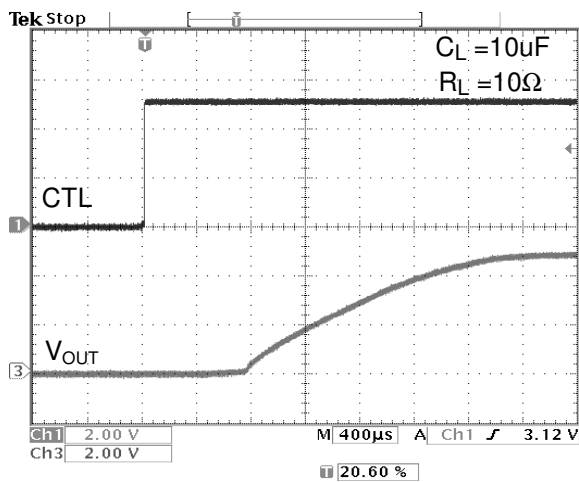
Fig. 15 Turn ON Time
