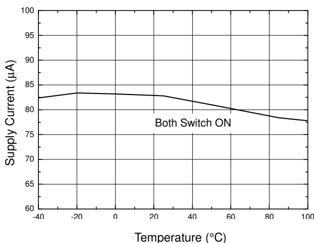
Fig. 5 ON State Current vs. Temperature
