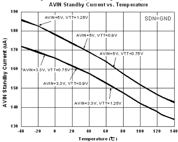
Fig.5 AVIN Standby Current vs. Temperature
