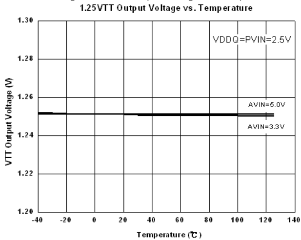
Fig.3 1.25VTT Output Voltage vs. Temperature
