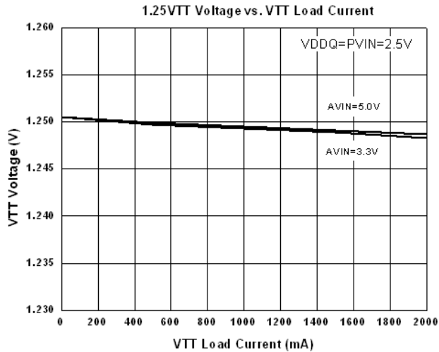
Fig.7 1.25VTT Voltage vs. VTT Load Current
